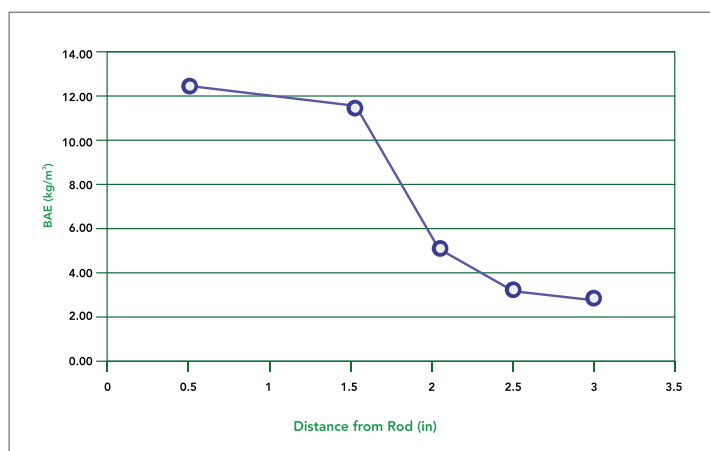
Boron Concentration as a Function of Distance from Cobra™ Rod Location
